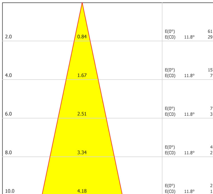
Distance [m] Cone Diameter [m] Illuminance [lx] — C0 - C180 (Half-value Angle: 23.6°)
